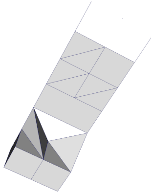
Fig. 1.23: Unstructured grid.
