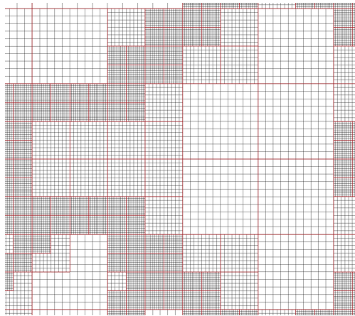
Fig. 1.22: AMR dataset.
