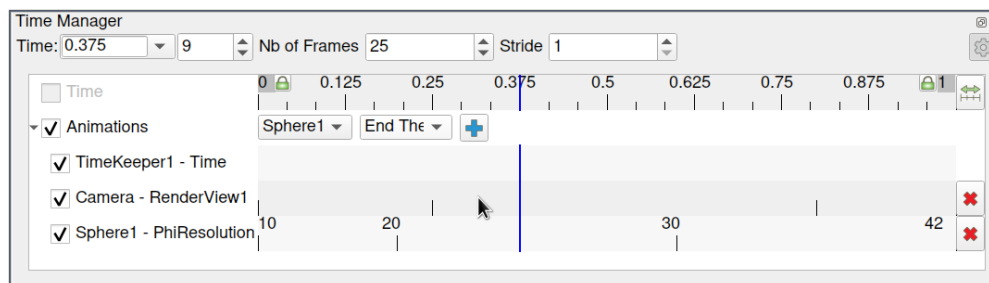
Fig. 1.111: Time Manager.
