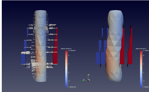
Fig. 1.85: The Warp By Vector filter can be used to displace points in original data shown on the left, using the displacement vectors (indicated by arrow glyphs Section 1.5.8) to produce the result shown on the right.
