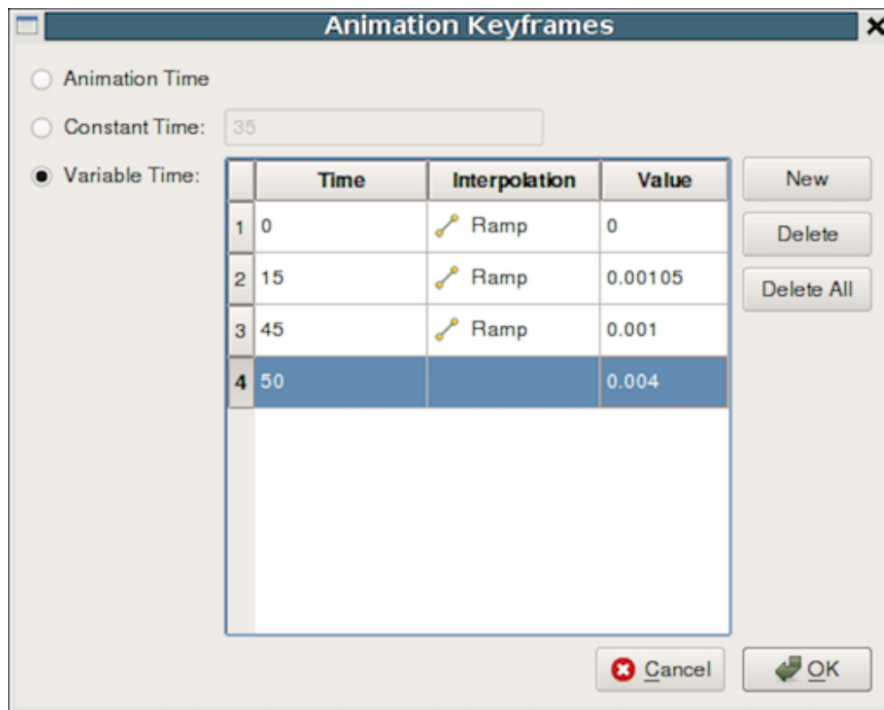
Fig. 1.117: Controlling Data Time with keyframes.
