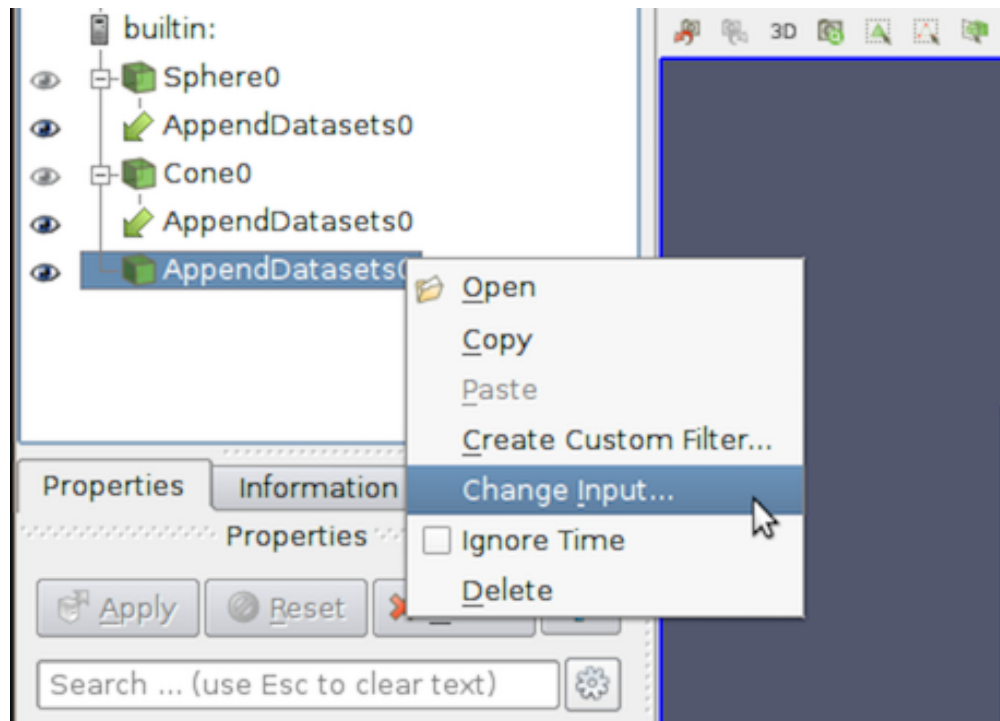
Fig. 1.76: The context menu in the Pipeline Browser showing the option to change inputs for a filter.
