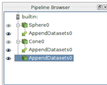
Fig. 1.74: The Pipeline Browser showing a pipeline with multiple input connections. The Append Datasets filter has two input connections on its only input port, Sphere0 and Cone0 .
