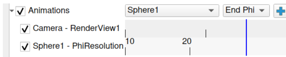
Fig. 1.112: Animation Tracks.
