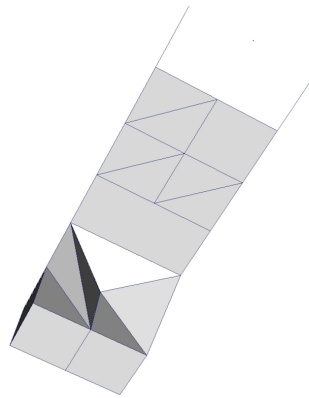
Fig. 1.26: Unstructured grid.
