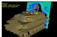
Fig. 4.1: ZSU23-4 Russian Anti-Aircraft vehicle being hit by a planar wave. Image courtesy of Jerry Clarke, US Army Research Laboratory.
