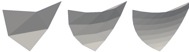
Fig. 1.42: A dataset made of quadratic tetra hedra displayed with 1, 2, and 3 levels of nonlinear subdivision.
