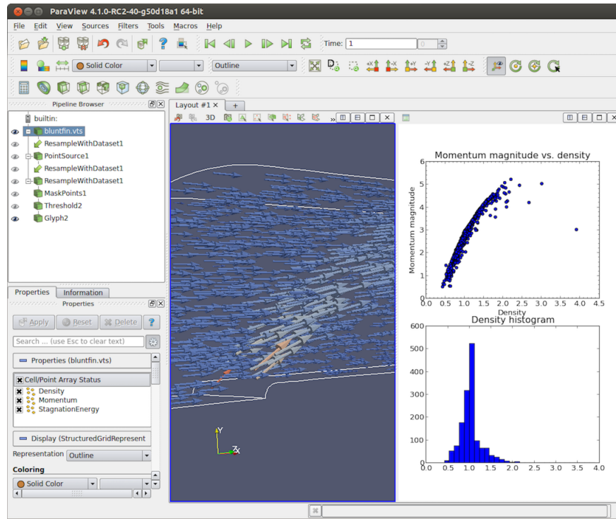
Fig. 1.52: paraview using Python View with matplotlib to display a scatterplot of momentum magnitude versus density (upper right) and a histogram of density (lower right) in the bluntnfin.vts dataset.
