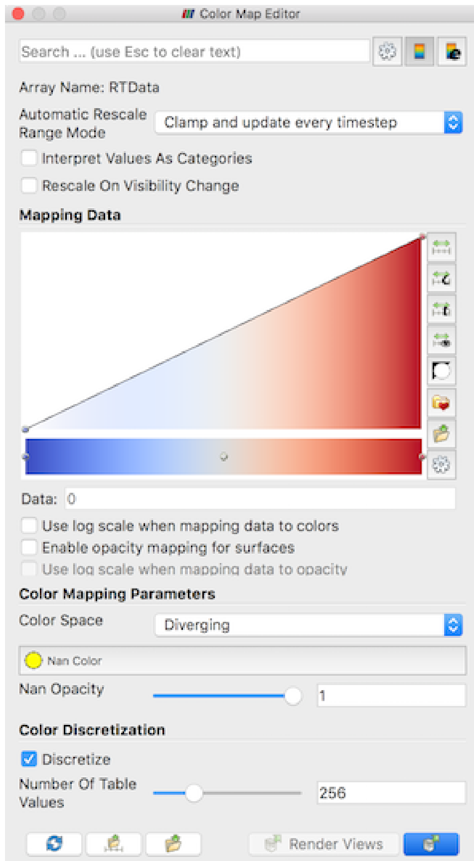
152 Fig. 2.4: Color Map Editor panel in paraview showing the major components of the panel. Chapter 2. Paraview Reference Manual
