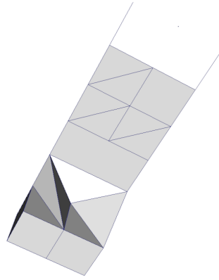
Fig. 1.26: Unstructured grid.
