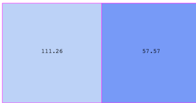
Fig. 1.21: Cell-centered attribute.
