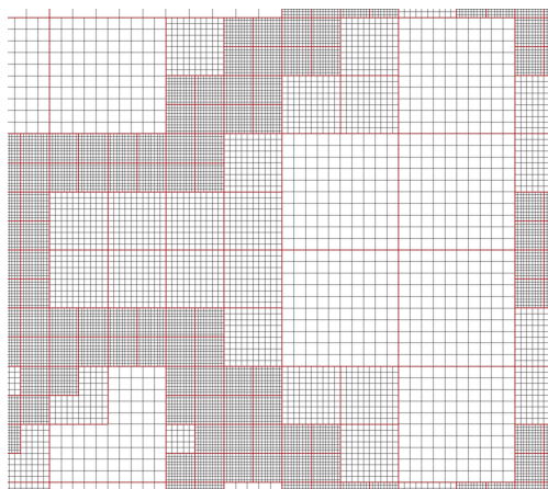
Fig. 1.25: AMR dataset.
