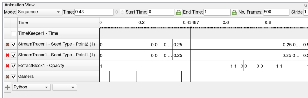
Fig. 1.103: Animation View.
