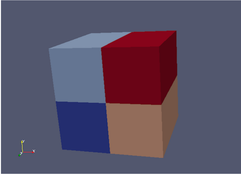
Fig. 2.27: Wavelet source processed by the D3 filter and colored by vtkProcessId array. Note how four regions of the image data are split evenly among the four processing cores when pvsrvr is run with mpirun -np 4 pvsrvr .
